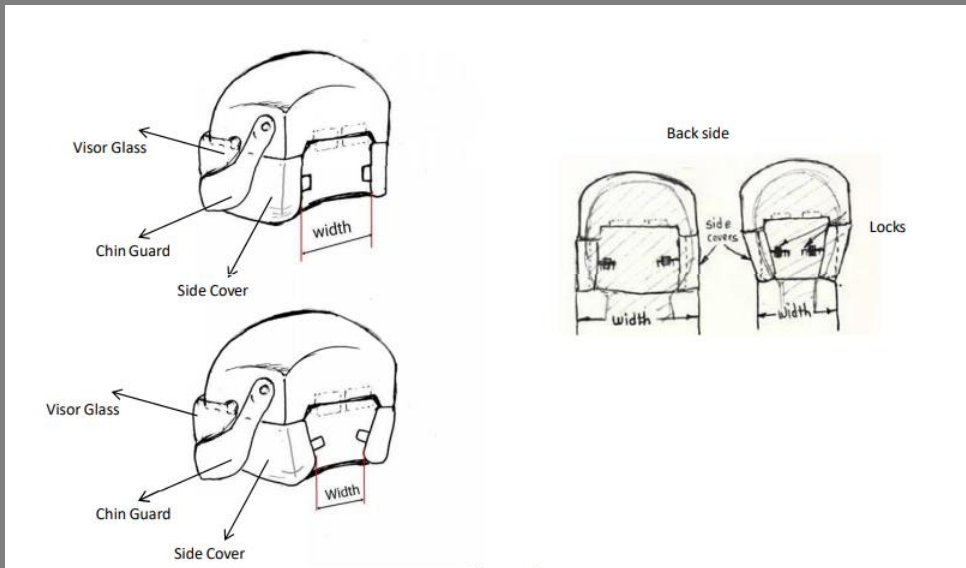
Size Adjusting Mechanism
